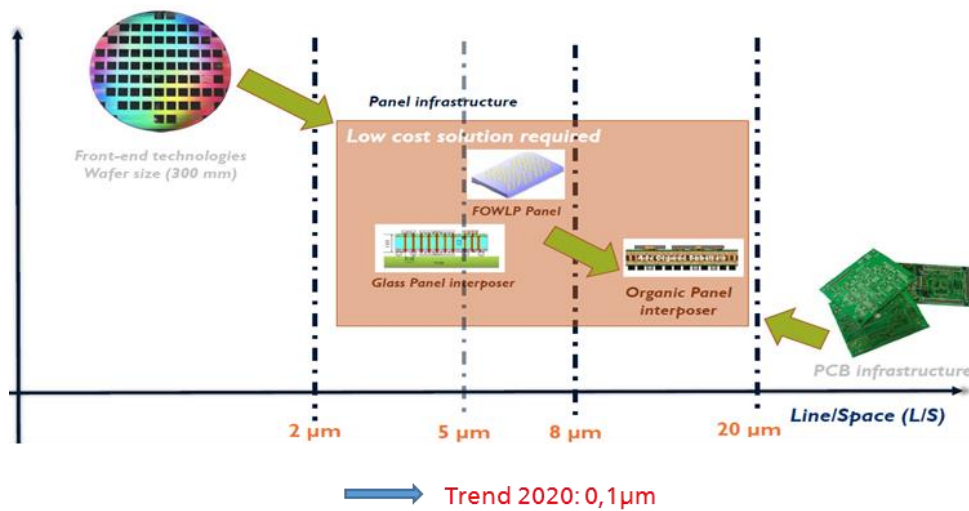
Figure 8 - The heterogeneous integration domain in electronic components merges the conventional PCB with the wafer level technologies (source: Fraunhofer IZM).
