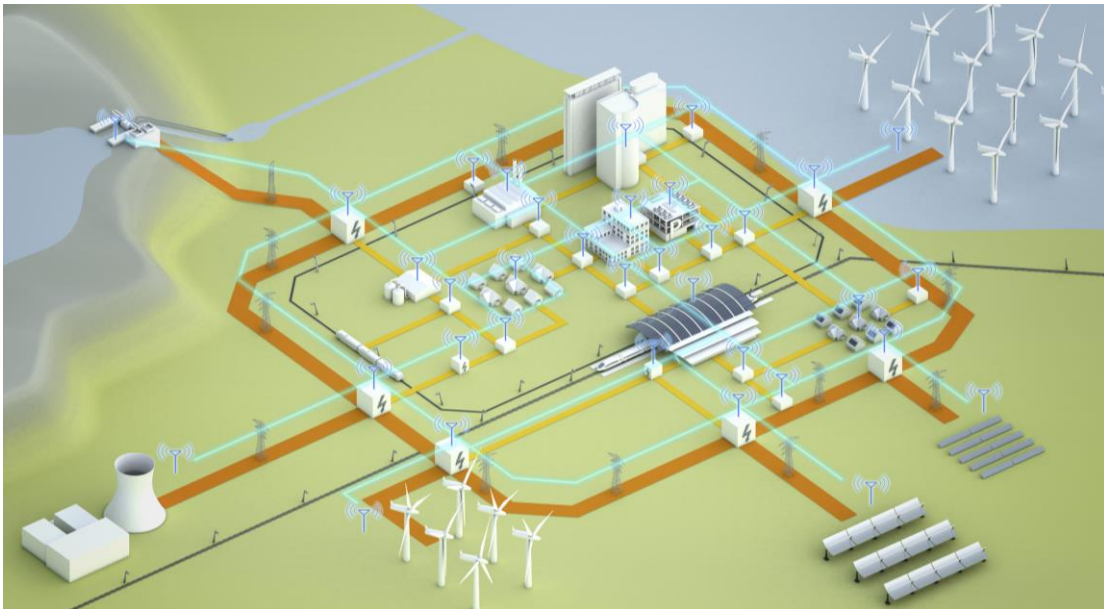
Figure 29 - Smart Energy landscape – from centralised to distributed (PV, wind, biogas, ...) generation and conversion, consisting of High/Medium Voltage grid (orange), Low Voltage grid (yellow) including Communication Network (aquamarine) linking producers and consumers down to regional and community level (source ECSEL MASP 2016 42 ).
