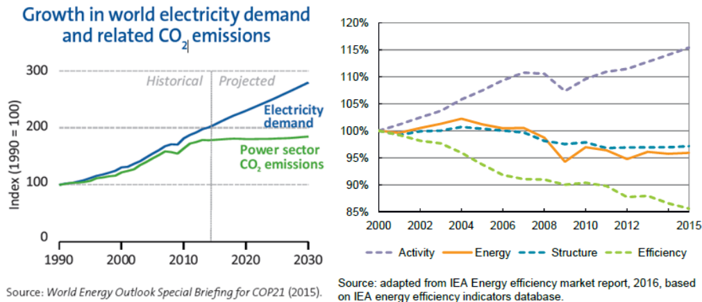
Figure 27 – Growth in world electricity demand and related CO 2 emissions
