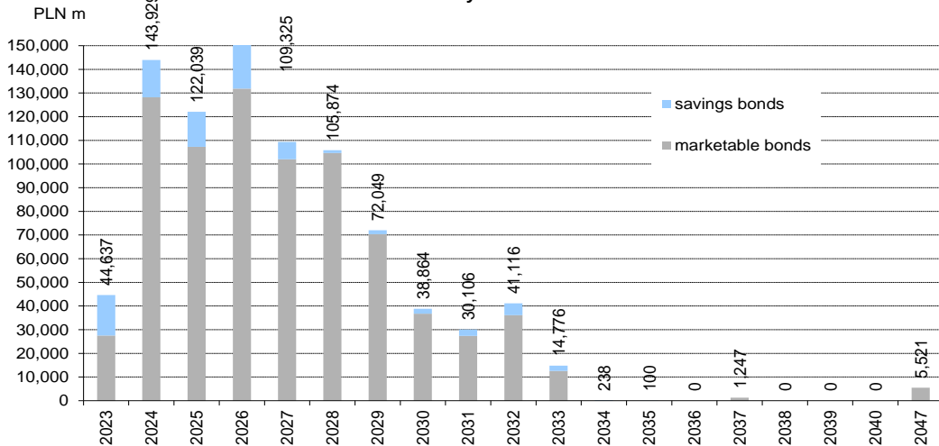
Maturity profile of the domestic Treasury securities debt as at the end of May 2023*
