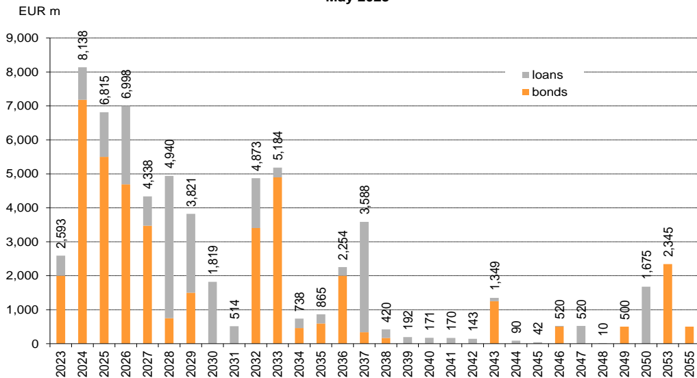
Maturity profile of the foreign debt (Treasury securities and loans) as at the end of May 2023
