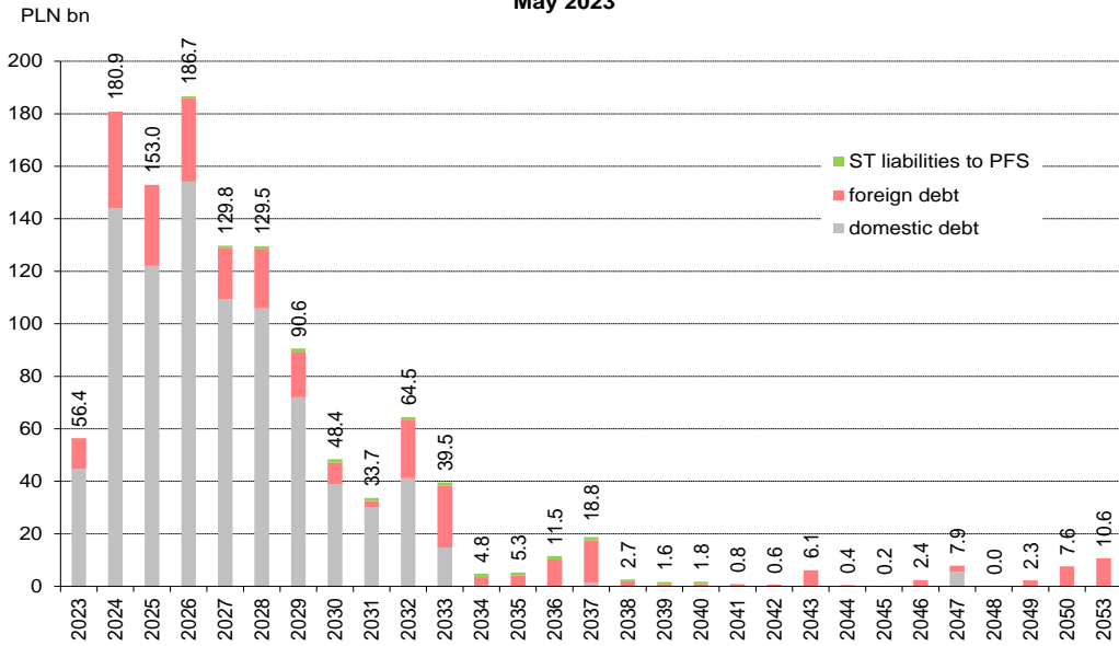
Maturity profile of the ST debt (Treasury securities and loans) as at the end of May 2023
