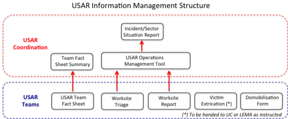
Figure 12: Information flow during core USAR operations
